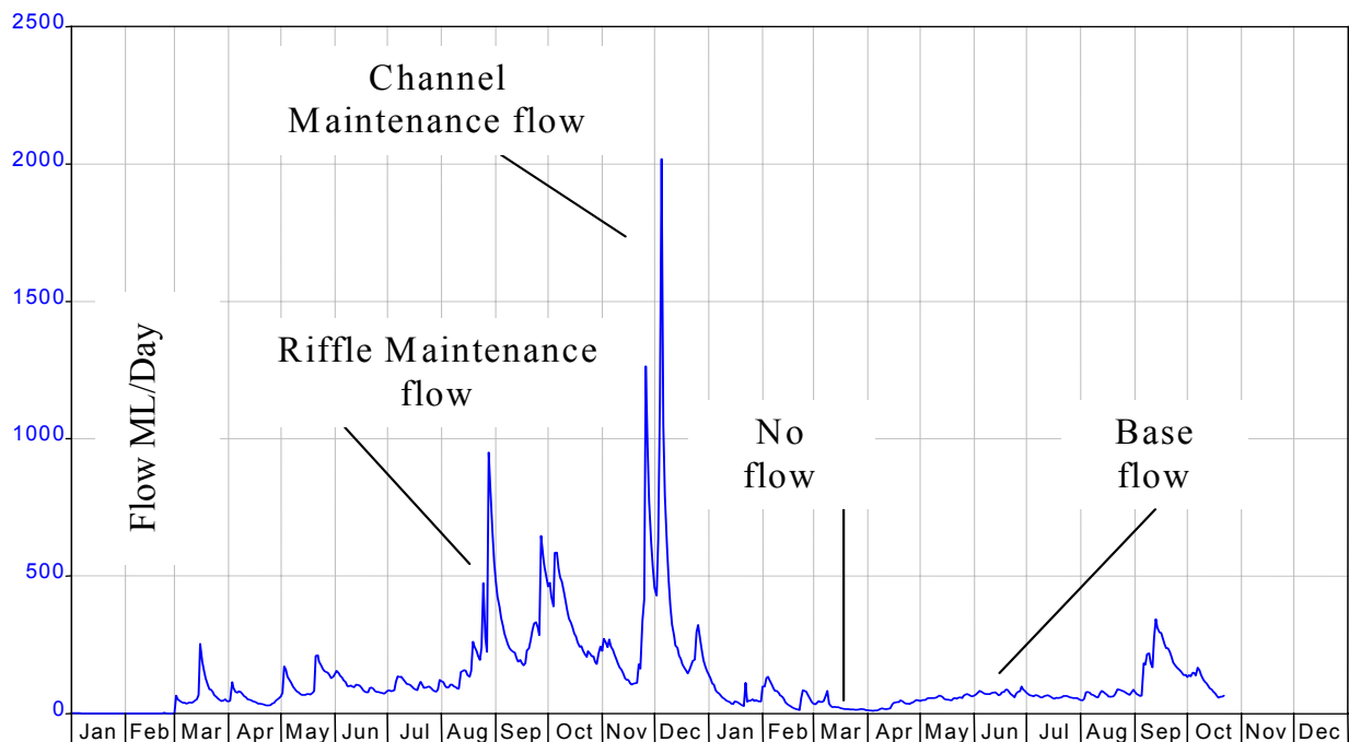
Figure 1: Flow at Lobbs Hole on the Murrumbidgee River near the ACT – NSW border over 2003-2004 illustrating flow variability and flow elements to be considered in an environmental flow regime.
